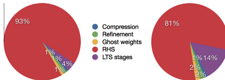
Fig. 15. Percentage of different stages in one simulation time step for the execution on 1 core (left) and 16 cores (right).
