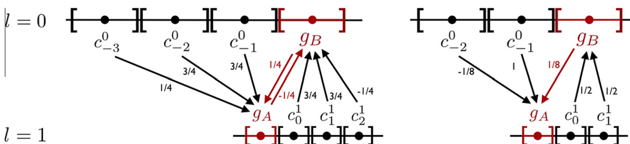
Fig. 1. Graph of the contributions for the reconstruction of the ghost g_A , with a resolution jump of 1 for the case of third-order b-spline wavelets (left) and third-order average interpolating wavelets (right). The arrows, and their associated weights, denote contributions from the grid points to the ghosts g_A and g_B . Both wavelets need the secondary ghost g_B to evaluate g_A , but average interpolating wavelets are more efficient as the evaluation of g_B does not depend on g_A (i.e. there is no loop in the graph).
