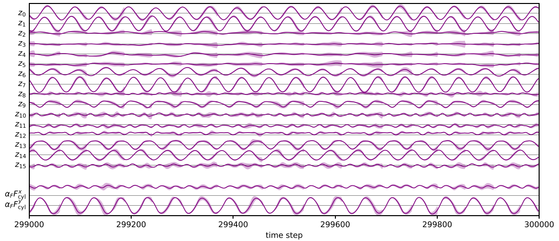
Fig. D.4. The trajectory \mathbf{z}(t) and \alpha_F \mathbf{F}_{cyl}(t) from the simulation from Section 5.1.1, as predicted by the ensemble. The solid line represents the ensemble mean prediction, and the faded region is the prediction uncertainty (the ensemble’s standard deviation). For clarity, the uncertainties are enhanced by 8\times . The numbers range between approx. -0.5 and 0.5 . See Appendix D.5.
