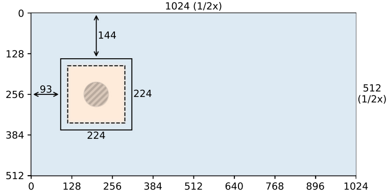
Fig. D.1. The geometry of the multiresolution autoencoder with resolution of AE_2 equal to 224 \times 224 . The solid inner box represents the subdomain that AE_2 operates on, the dashed line the distance d^r = 22 from the inner subdomain boundary (where \beta^{(1)} = \beta^{(2)} = 0.5 ). Colors represent the blending contributions ( \beta^{(1)} > 0.5 marked as blue, \beta^{(2)} > 0.5 with orange), and circle the cylinder. (For interpretation of the references to color in this figure legend, the reader is referred to the web version of this article.)
