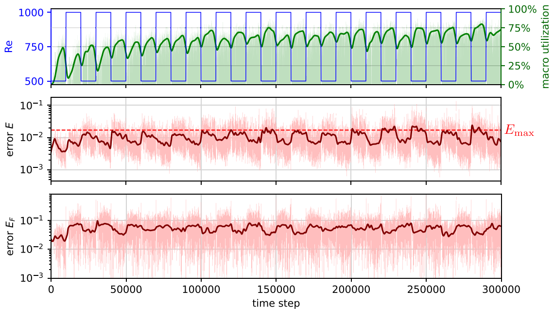
Fig. D.5. AdaLED performance on a flow behind cylinder simulation for Re(t) \in \{500, 1000\} , analogous to Fig. 9. Top: Reynolds number Re(t) profile and the macro utilization \eta . Middle and bottom: validation errors of the velocity ( E , Eq. (13)) and force on the cylinder ( E_f , Eq. (14)). The per-step errors (faded red) alternate between low values at the beginning of the macro-only stage and higher errors at the end of the macro-only stage. (For interpretation of the references to color in this figure legend, the reader is referred to the web version of this article.)
