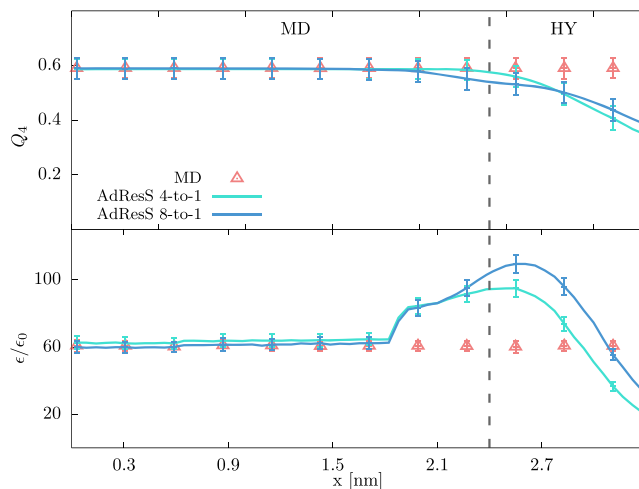
FIG. 9. Local tetrahedral order parameter Q_4 (top) and dielectric permittivity (bottom) as a function of x coordinate of the simulation box.
