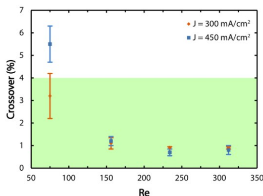
Figure 6. GC results for a set of flow rates and current densities. The green zone shows the safe region for the purity of the gas. By increasing the flow rate, the separation of gas bubbles based on the inertial fluidic forces come into effect which leads to almost pure streams of the gases at the outlets.
