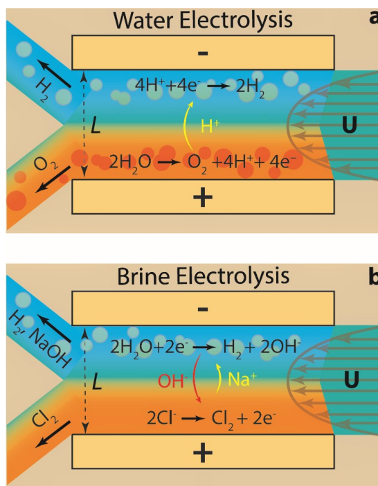
Figure 2. The membrane-less reactor of this study is tested for two electrochemical reactions: a) water electrolysis and b) brine electrolysis. The flow rate in both cases should be fast enough to minimize the crossover due to the diffusion of dissolved gases and provide large inertial forces to keep the gas bubbles of each side away from the channel's centreline. In the brine electrolysis, the convective transport of hydroxide ions should also dominate its diffusion towards the anode, which can initiate oxygen evolution as a competing reaction for chlorine evolution.
