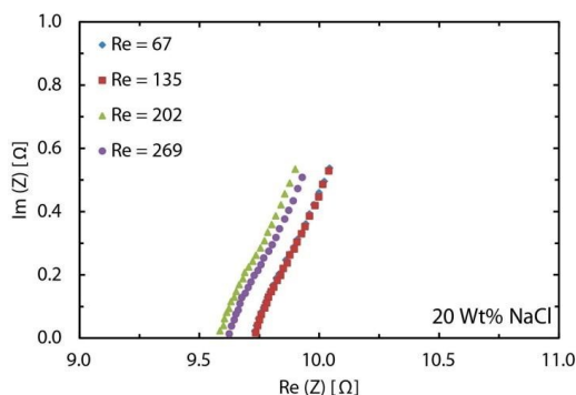
Figure 11. PEIS measurements for the Chlor-Alkali reaction with 20 Wt% NaCl electrolyte at different flow rates. Similar to the water splitting, better ohmic contacts can provide more than 300 mV reduction in the cell potential when working at around 700 mA/cm 2 .
