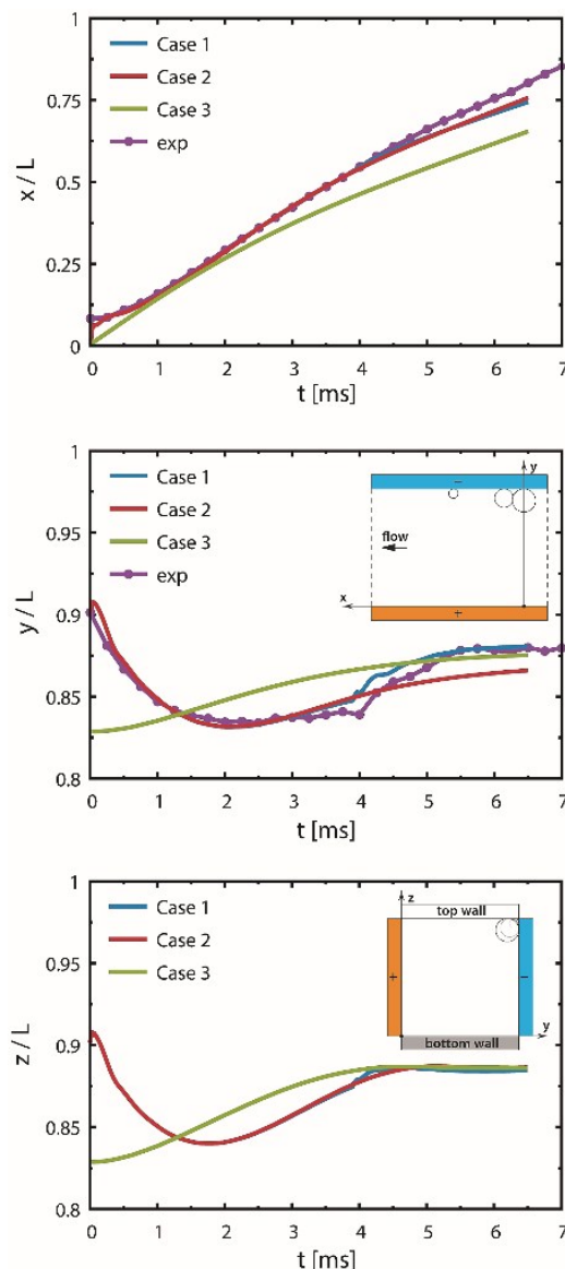
Figure 8. Trajectory of the newly formed bubble from simulations for various initial configurations. The curves track the position of the bubble center for three cases in the streamwise ( x -axis), in between the electrodes ( y -axis) and in the depth ( z -axis) with time. The inset sketches of the middle and bottom figures illustrate the coordinate system from two views. Gravity acts towards the bottom wall (opposite to the z -axis). Case 1: two bubbles located upstream and a smaller bubble downstream as shown in Figure 7, jump-off at t = 1.5 ms and rapid return at t = 4 ms after coalescence with the smaller bubble. Case 2: two bubbles, slower return caused by the inertial force and buoyancy. Case 3: a single bubble placed at a distance from the corner to reproduce conditions after the jump-off without having the disturbances in the flow caused by the coalescence. Experimental data (exp) correspond to Case 1.
