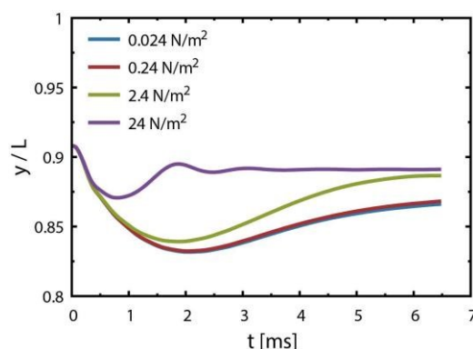
Figure 9. Trajectory of the newly formed bubble from simulations of Case 4, showing the effect of the Marangoni force. The curves follow the position of the bubble center in between the electrodes (y-axis) with time. Initial configuration consists of two bubbles placed at the corner as in Case 2. Various surface tension gradients are imposed within a boundary layer of thickness 0.1 mm starting from the electrode surface at y/L = 1 towards the center of the channel. The Marangoni force contribution is minimal compared to the inertial forces for small surface tension gradients.
