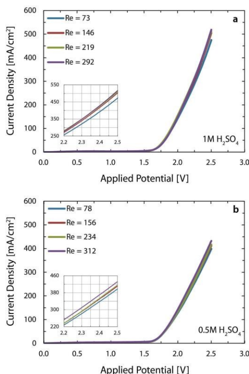
Figure 4. Polarization curves of the water splitting reaction with 1M (a) and 0.5M (b) sulfuric acid electrolytes for different flow rates. In both cases, going from the lowest to the highest Re increases the current density by around 10% thanks to the lower volume fraction of the gases in the cell and smaller sizes of detached bubbles. The performance of the cell is similar to the state-of-the-art alkaline electrolyzers but with more dilute and safer electrolytes and at room temperature. The inset provides a detailed view of the data above 2.2V.
