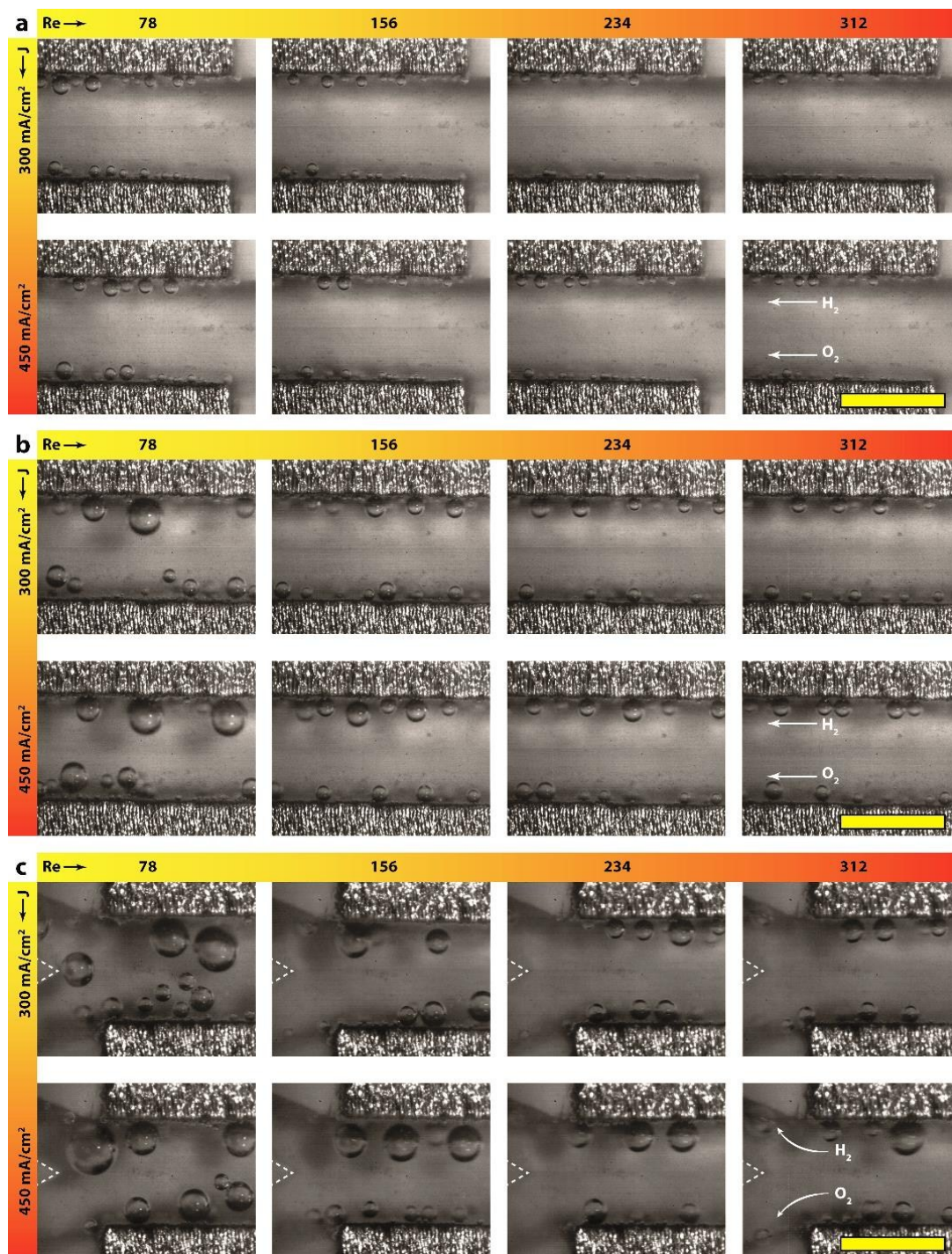
Figure 3. Snapshots of the upstream (a), midstream (b), and downstream (c) regions of the electrolyzer: In general, the volume fraction and average size of bubbles increase with decreasing flow rate or increasing the current density. At low flow rates, some bubbles depart from the walls and move towards the center since the inertial forces are not strong enough. This phenomenon increases the crossover rate at these conditions as quantified by the Gas Chromatography (GC) results. The separating wedge is highlighted with a dashed triangle for better clarity in the downstream figures. The yellow scale bars at the corners are 1 mm in size.
