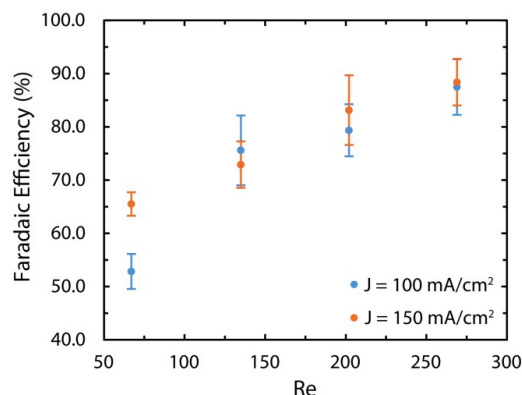
Figure 12. The Faradaic efficiency of the brine electrolysis at different current densities and flow rates measured with the colorimetry technic. The most likely reason for the low efficiency at low flow rates is the loss of \text{Cl}_2 in gaseous form. The colorimetry method can only measure the amount of dissolved chlorine. This explanation is corroborated by the pH measurements provided in the supporting information that indicate Faradaic efficiencies of more than 88% for all sets of current densities and flow rates.
