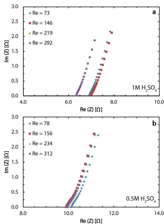
Figure 5. PEIS measurements for the water splitting reaction with 1\text{M} (a) and 0.5\text{M} (b) sulfuric acid electrolytes at different flow rates. The obtained ohmic losses are larger than the calculated values from Ohm's law since the losses at the contacts between the electrodes and the power source are measured here in addition to the solution resistance. Better ohmic contacts can provide 200 \text{ mV} reduction in the cell voltage when working at around 400 \text{ mA/cm}^2 .
