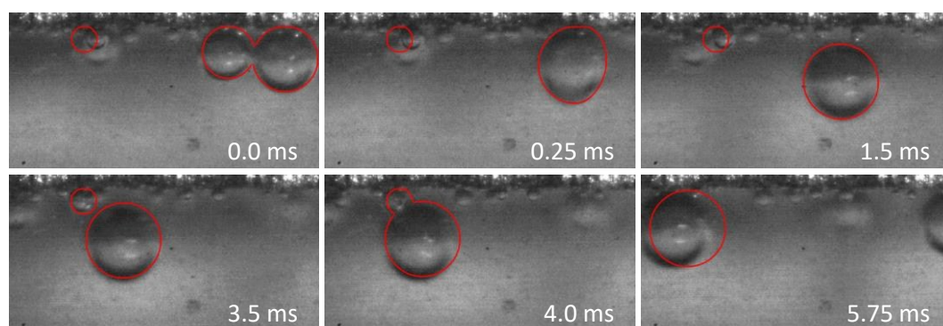
Figure 7. Snapshots from the experiment at Re = 234 overlaid by projections of the bubble shapes from the simulation (red lines). The flow direction is from right to left. All three bubbles are initially placed at the channel corner, with one smaller bubble present further downstream. Coalescence of the larger bubbles causes the jump-off at t = 1.5 ms followed by a rapid return towards the electrode at t = 4.0 ms after coalescence with the pinned bubble.
