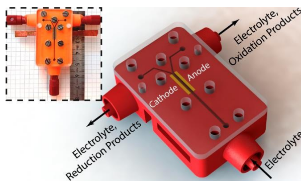
Figure 1. Schematic illustration of the electrolysis cell: The main body (in red) is 3D printed with stereolithography technology. The electrodes (in yellow) are pressed into the devised slots and the assembly is covered by a transparent PMMA plate. A flexible sealing film is sandwiched in between this plate and the 3D printed part to prevent leaking. The inset shows the final assembled device with attached fluidic connectors.
