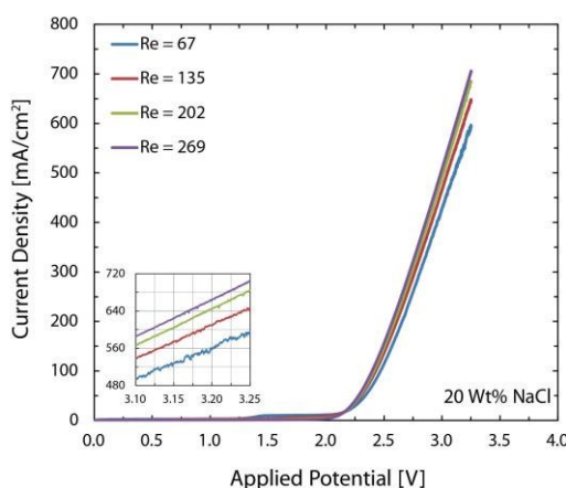
Figure 10. Polarization curves of the Chlor-Alkali reaction with 20 Wt% NaCl electrolyte for different flow rates. By moving from the lowest to the highest Re enhances the current density by approximately 20% thanks to the lower gas volume fraction and lower catalyst coverage by nucleating bubbles. The performance of the cell at room temperature is similar to the state-of-the-art cells that operate at around 90°C. The inset provides a detailed view of the data above 3.1 V.
